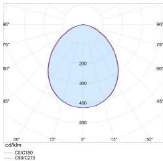
6721.405.V3.LM11 54 W MATTALASI
