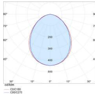
6741.405.V3.LM11 71 W MATTALASI
